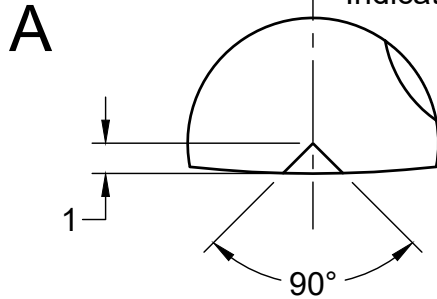
DETAIL A SCALE 4:1 Indicator Notch
